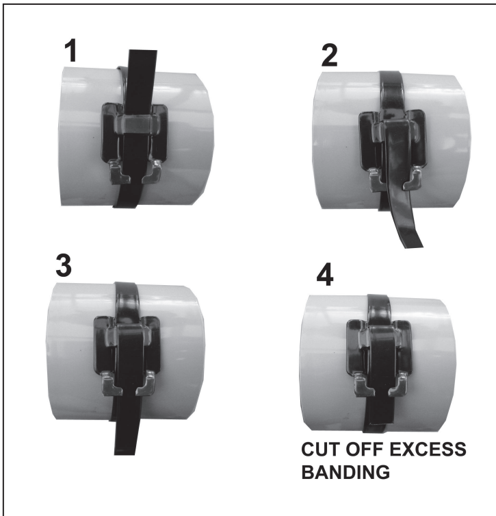
LOCKING BAND CLAMP INSTALLATION FIGURE THREE
